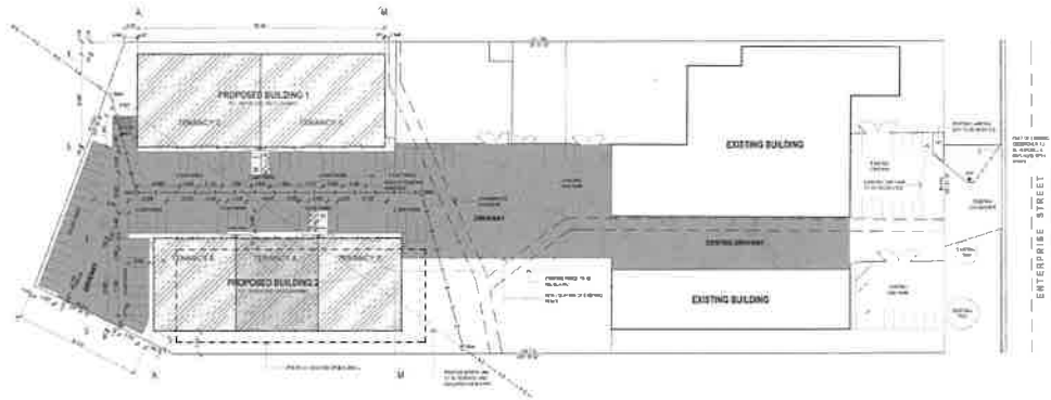
PROPOSED SITE PLAN SCALE 1:500
